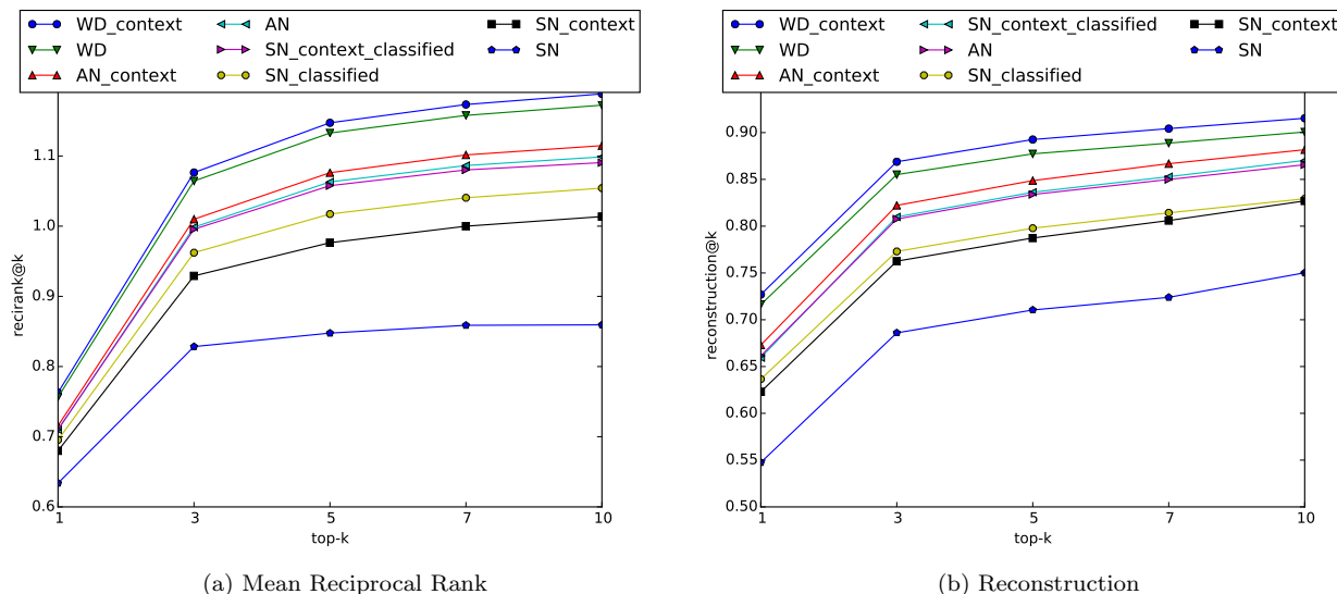
Figure 3: Evaluation Measures
