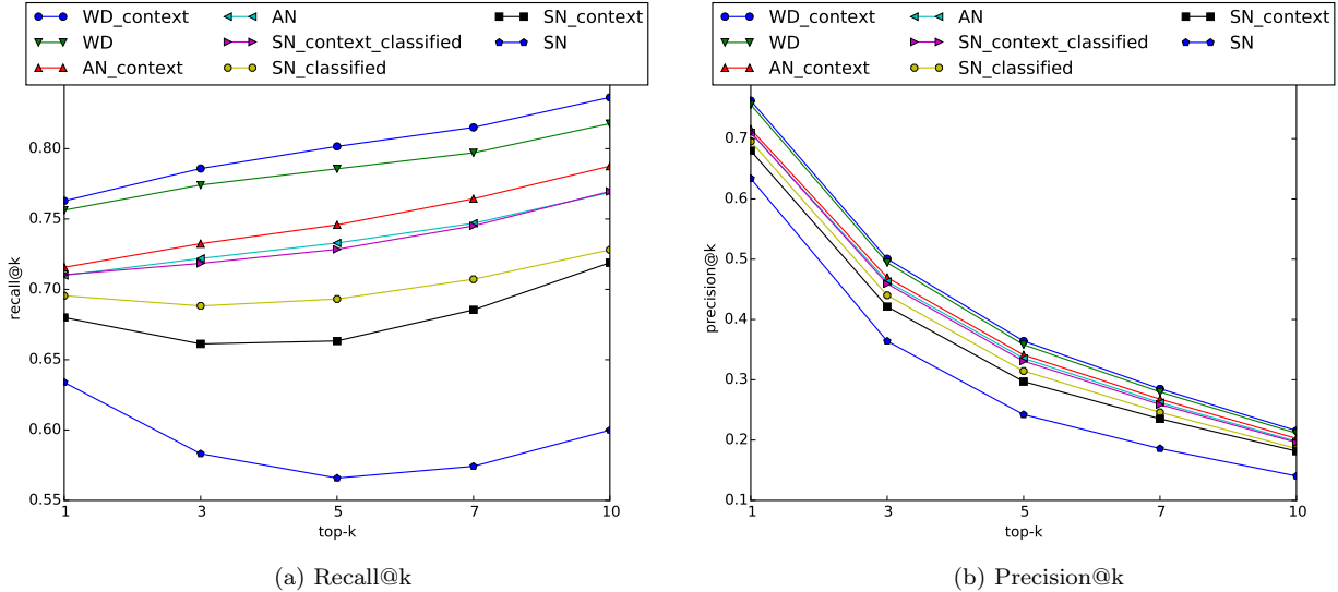
Figure 2: Evaluation Measures
