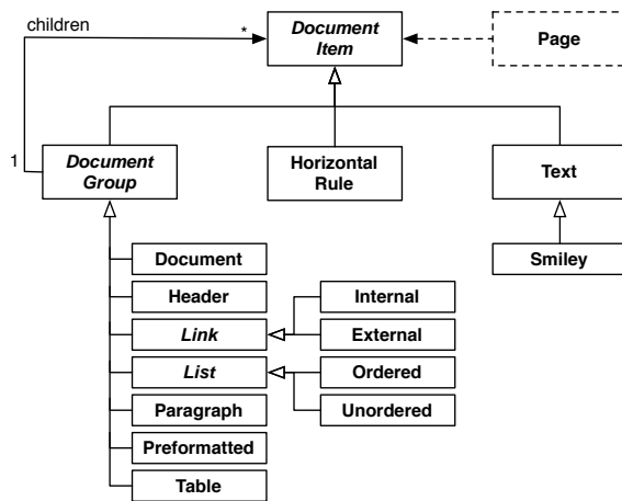
Figure 5: The document hierarchy: a simple composite.
